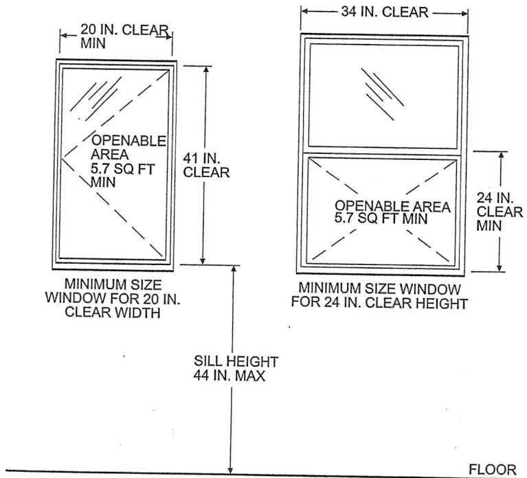
Figure R310.1 EMERGENCY ESCAPE AND RESCUE WINDOW
